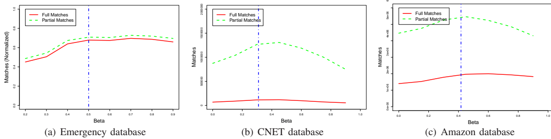
Fig. 8. Effect of \beta_1 in the Bernoulli Model.
