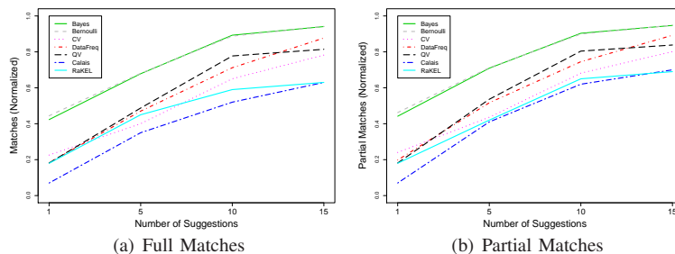
Fig. 5. Number of Full and Partial Query Matches in Emergency DataSet.
