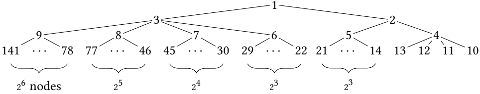
Fig. 6. The top three levels of T_\infty . Each node i has 2^{i-p(i)} children, where p(i) is the parent of i (exc. p(1) = 0 ). The merge tree T_2^N (Figure 5) consists of these three levels, with each node i given weight 2^{N-p(i)} , so the nodes with weight 2^{N-i} are the 2^{i-p(i)} children of node i , and their total weight equals the weight of node i . Note that the label of a node in the merge tree is its weight, and the merge tree of Figure 5 is T_2^{18} .
