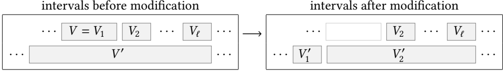
Fig. 10. Replacing intervals V and V' by V'_1 and V'_2 (proof of Theorem 4.1).
