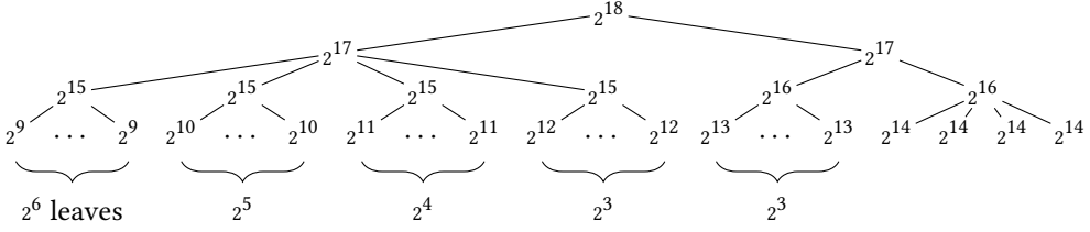
Fig. 5. The “merge tree” for an execution of the Adaptive-Binary algorithm (Figure 3). The input sequence starts with m = 132 inserts I_1, I_2, \dots, I_{132} — one for each leaf, of weight equal to leaf’s label. It continues with 2^{16} - 132 empty inserts ( I_t = \emptyset ). At each time t = 2^9, 2^{10}, 2^{11}, \dots, 2^{17} (during the empty inserts) the algorithm merges all components of weight t to form a single new component, their parent. In this way, the algorithm builds a component for each node, with weight equal to the node’s label. At time t = 2^{17} the final component is built—the root, of weight 2^{18} , containing all items. The algorithm merges each item four times, so pays build cost 4 \times 2^{18} .
