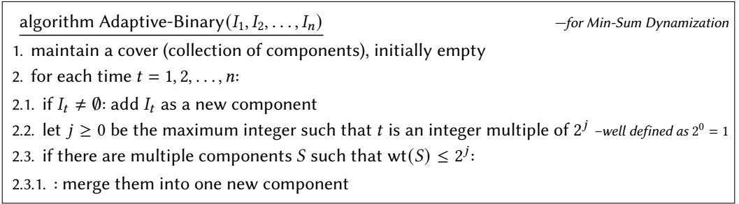
Fig. 3. A \Theta(\log^* m) -competitive algorithm for Min-Sum Dynamization (Theorem 2.1).
