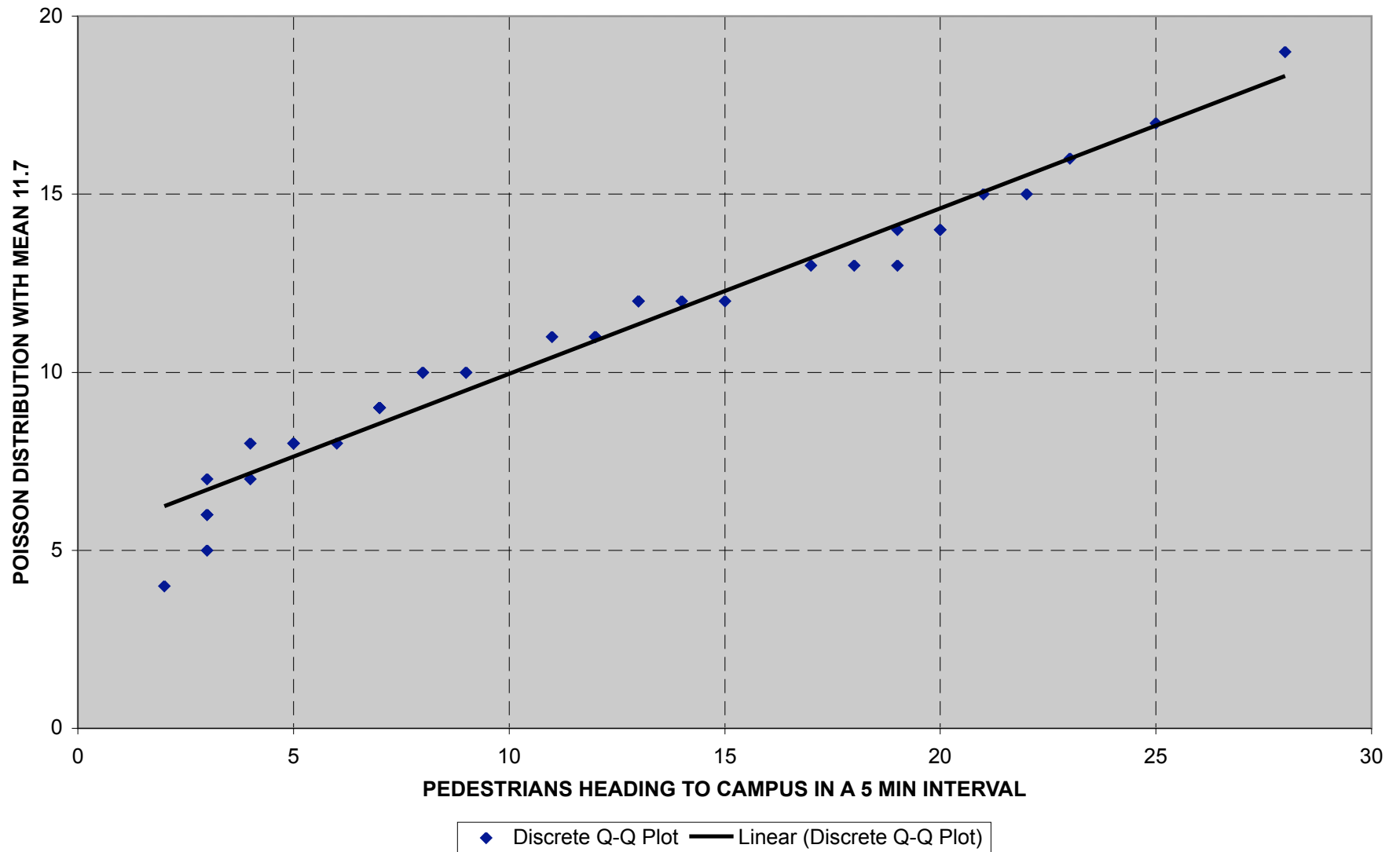
Figure 6: Discrete Q-Q Plot of Pedestrian Counts vs. Poisson Distribution
