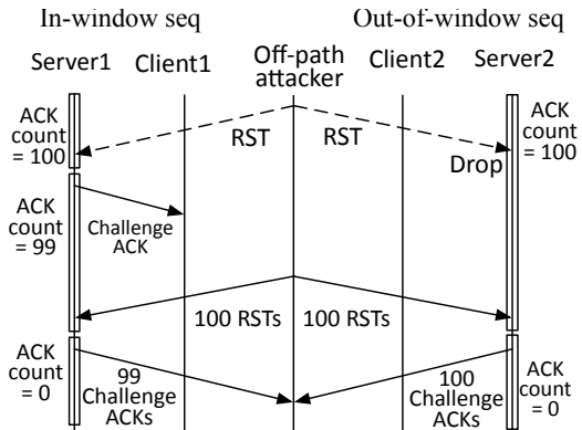
Figure 2: An illustrative TCP Side-Channel Vulnerability.
