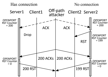
Figure 7: Reset counter based side channel example (Vulnerability 1, FreeBSD)
