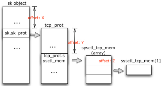
Offset chain: sk-(offset:X)-load:type1-(offset:Y)-load:type2-(offset:Z)-load:type3
