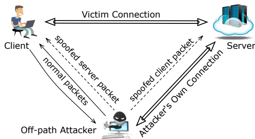
Figure 1: Threat model
