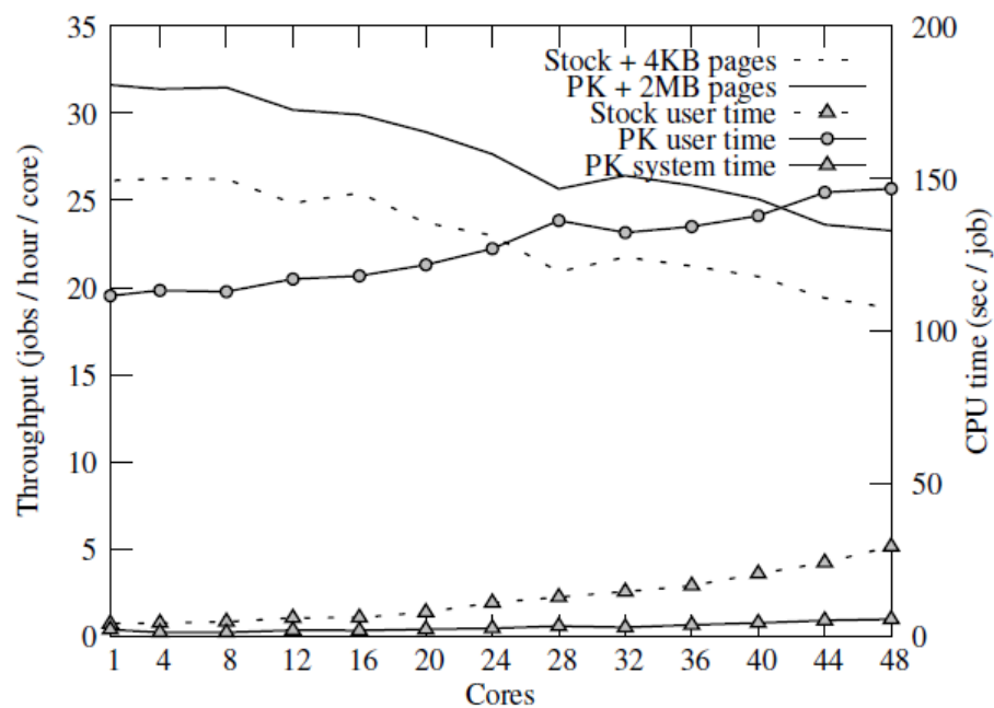
Figure 11: Metis throughput and runtime breakdown.
