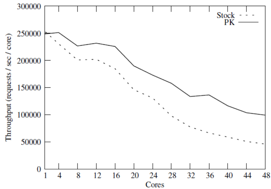
Figure 5: memcached throughput.
