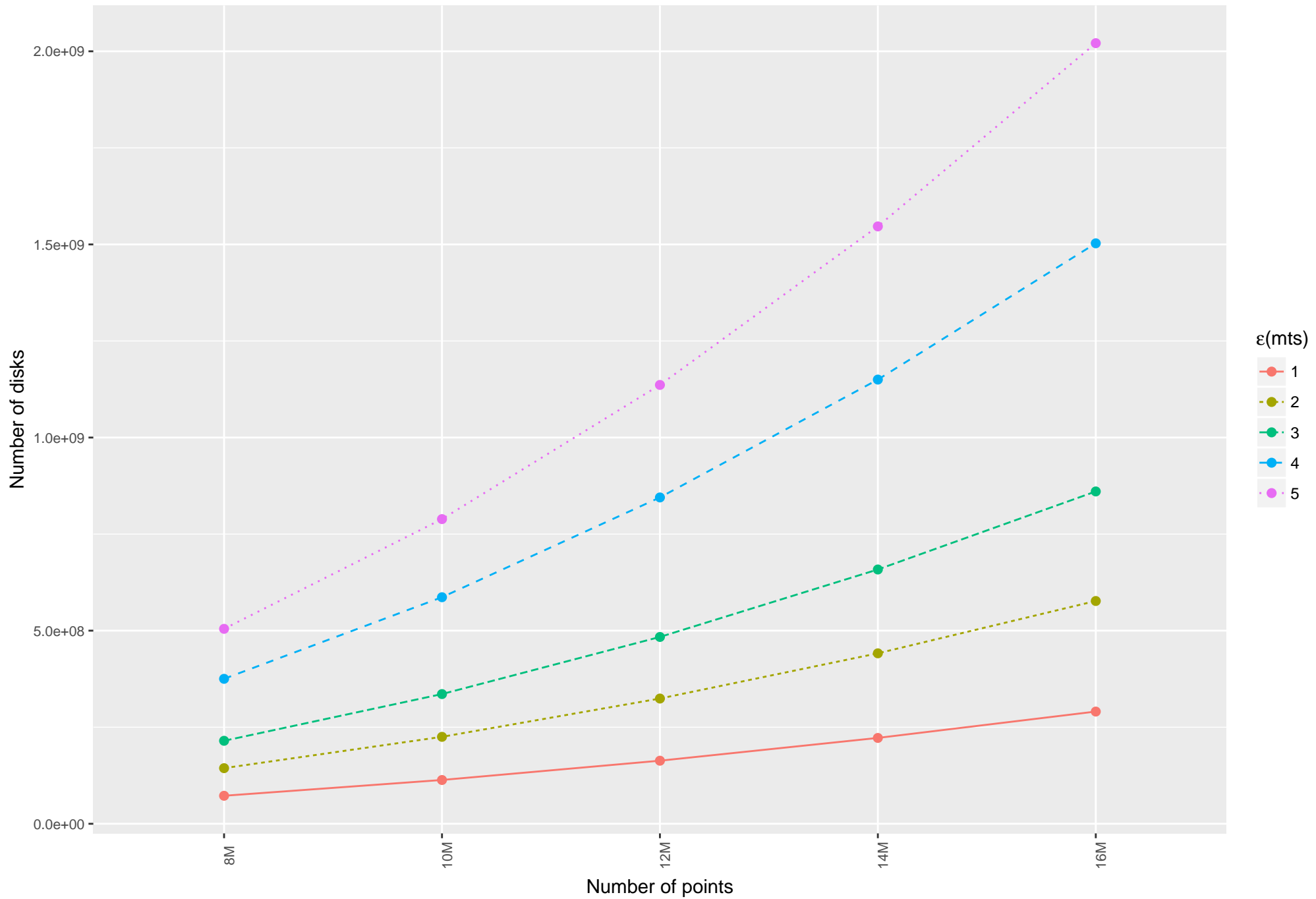
Number of disks by \epsilon (radius of disk in mts) in Cologne dataset.
