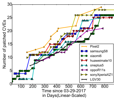
Figure 13: Different OEM vendor comparison
