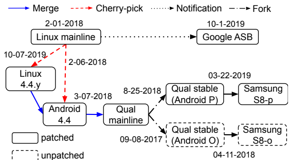
Figure 16: Case study: CVE-2019-2215
