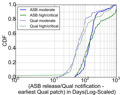
Figure 18: Notification delays of Qualcomm CVEs (by severity)
