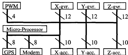
Figure 2. Bus structure for GPS Navigation System.
