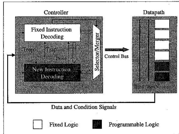
Figure 3. Dynamic-decode Architecture
