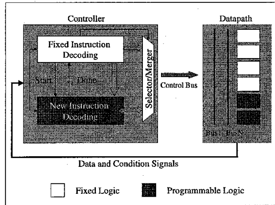
Figure 2. Static-decode Architecture
