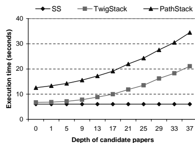
(a) Execution time (b) Number of partial solutions Figure 17: PathStack versus TwigStack on a real data set
