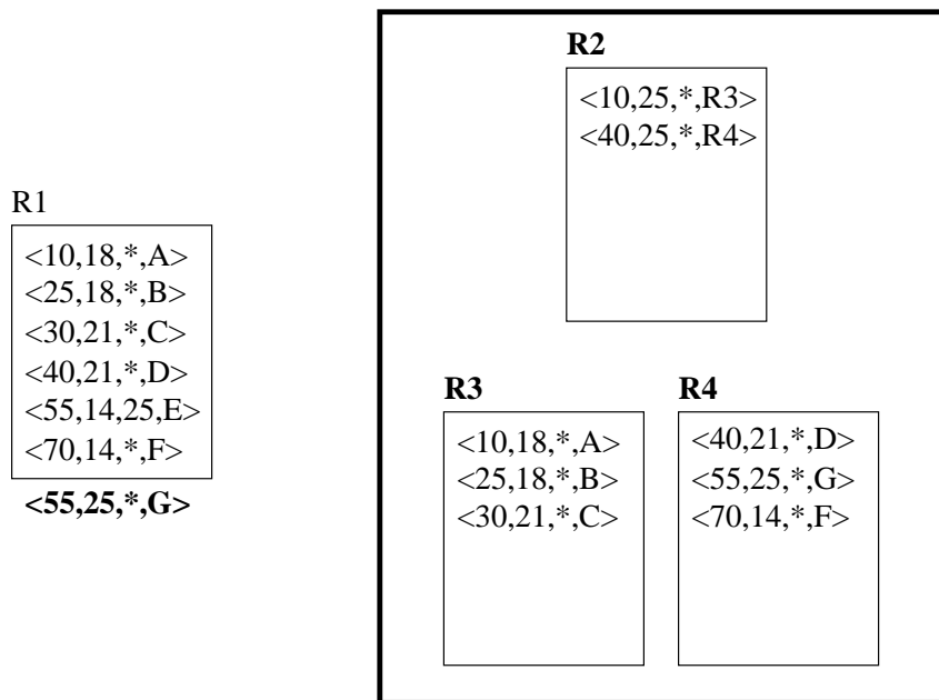
Fig. 4: Key split after strong version overflow of root block R1
