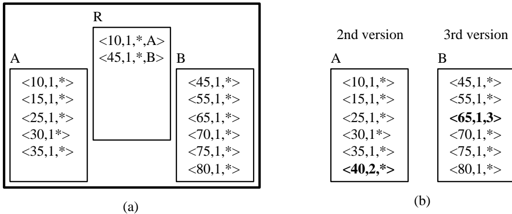
Fig. 1: Development of the multiversion B-tree up to the 3rd version
