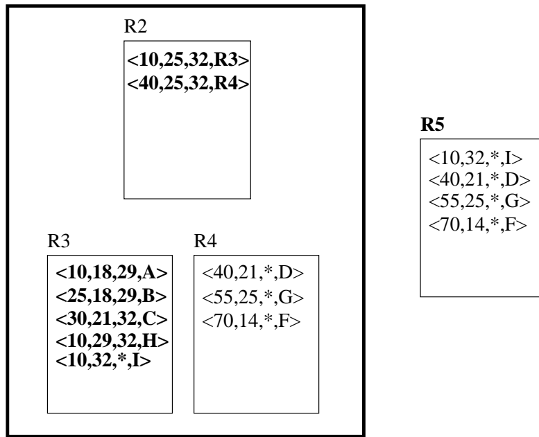
Fig. 5: Weak version underflow of root block R2
