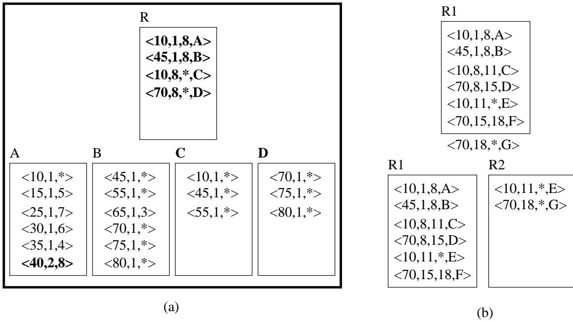
Fig. 3: (a) Structural changes after weak version underflow of block A and (b) Creation of two roots R1 , R2 by version split of root block R1
