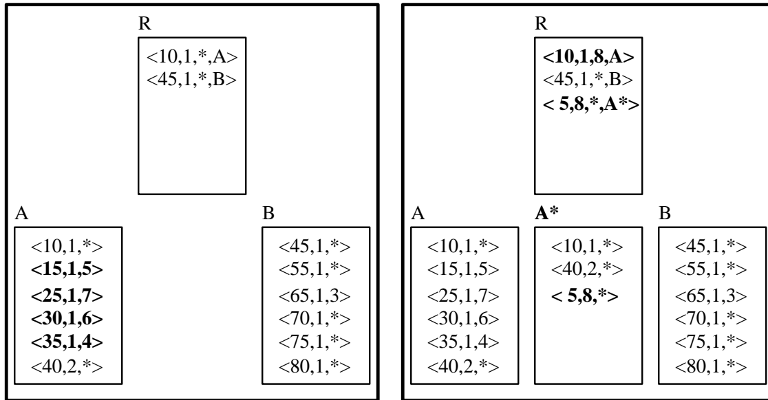
(a) The 7th version of the multiversion B-tree and (b) the multiversion B-tree after version split of block A
