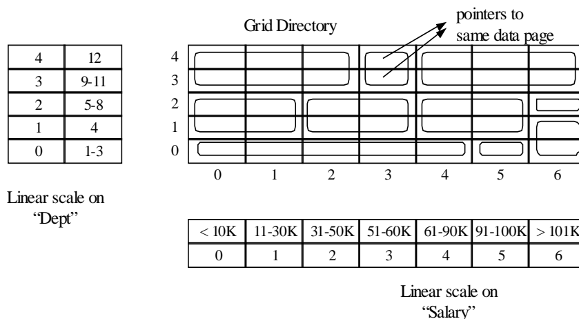
Figure 1. A Grid File.
