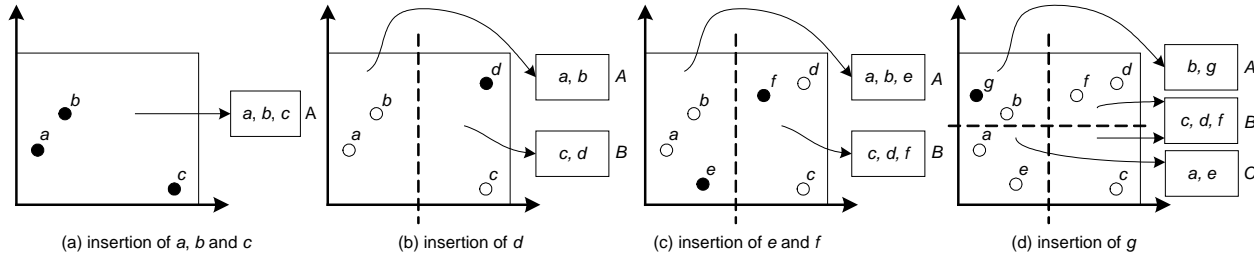
Figure 2. Insertions in the Grid File.
