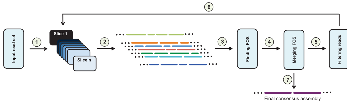
Fig. 1. SLICEMBLER's pipeline: First, the input reads are partitioned into smaller slices (1). Each slice is assembled individually (2), and the resulting assemblies are merged by a 'majority voting' process (3, 4). Before repeating these steps, any read in the input that maps to the consensus assembly is removed (6). When no further merging is possible, the final consensus assembly is produced (7)
