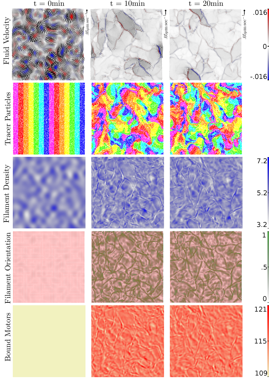
FIG. 6.2. Emergence of ordered subregions in the filament-motor-fluid system, depicted at t = 0 (first column), t = 10 min (second column), and t = 20 min (third column). First row: \mathbf{u}(\mathbf{x}, t) , with vorticity plotted in color (units of \text{s}^{-1} ). As the simulation proceeds, the fluid subregions form vorticity bands at their boundaries with zero vorticity in their interiors. Second row: tracer particles show fluid mixing. Third row: \Psi_{\text{spatial}}(\mathbf{x}, t) in \mu\text{m}^{-2} defined in Eq. (6.2). Fourth row: eigenvectors of \mathbf{N}(\mathbf{x}, t) (red lines) and S(\mathbf{x}, t) (green field) given in Eqs. (6.3)-(6.4). Fifth row: \mathcal{M}_b^{\text{tail}}(\mathbf{r}_0, t) in \mu\text{m}^{-2} defined in Eq. (6.5). At t = 0 , the density of filaments is perturbed in space and orientation according to Eq. (6.1), while the bound motor density is uniform. The parameters are L = 125\mu\text{m} , l = 1\mu\text{m} , \mu = 0.12\text{pNs}/\mu\text{m}^2 , \varepsilon = 5 \cdot 10^{-4} , N = 2 \cdot 10^4 , N_m = 3 \cdot 10^6 , k_{\text{on}} = 1\text{s}^{-1} , k_{\text{off}} = 0.5\text{s}^{-1} , D_{t,\parallel} = 0\mu\text{m}^2\text{s}^{-1} , D_r = 0\text{s}^{-1} .
