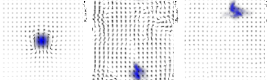
FIG. 6.1. Evolution of the velocity field and filament density for a clump of locally aligned filaments with uniform bound motor density, depicted at t = 0\text{s} , t = 50\text{s} , and t = 150\text{s} . The parameters are L = 125\mu\text{m} , l = 1\mu\text{m} , \varepsilon = 5 \cdot 10^{-4} , N = 2 \cdot 10^4 , N_m = 3 \cdot 10^6 , k_{\text{on}} = 0.5\text{s}^{-1} , k_{\text{off}} = 0.5\text{s}^{-1} . The dimensionless diffusion parameters to D_{t,\parallel} = 2.5 \cdot 10^{-3} and D_r = 2.5 \cdot 10^{-5} .
