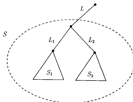
Fig. 3. Inductive proof.
