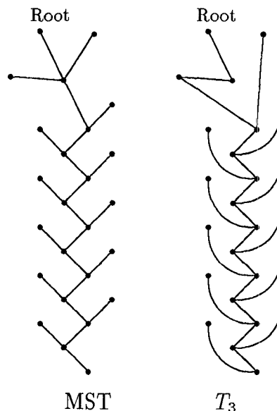
Figure 5: Bad example for algorithm in Fig. 2.
