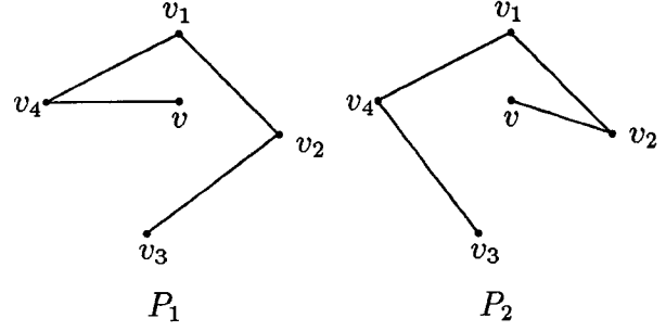
Figure 4: T_3 , four children
