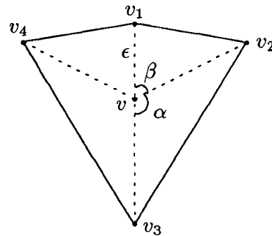
Figure 9: Figure to illustrate degree four case.
