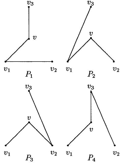
Figure 7: T_4 , three children
