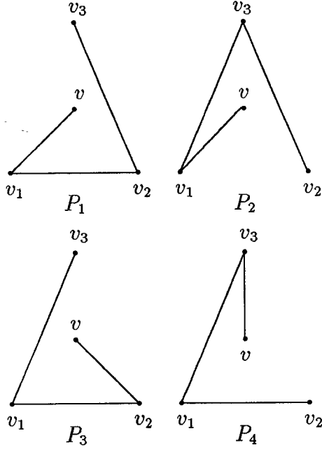
Figure 3: T_3 , three children
