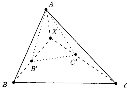
Figure 1: Shrinking to obtain canonical form
