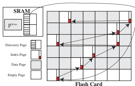
Fig. 3. Overview of the MicroHash Structure. While a node senses data from its environment it also creates index entries that point to the respective data stored on the flash media. When a node needs to evaluate some query, it uses the index records to quickly locate the desired data.
