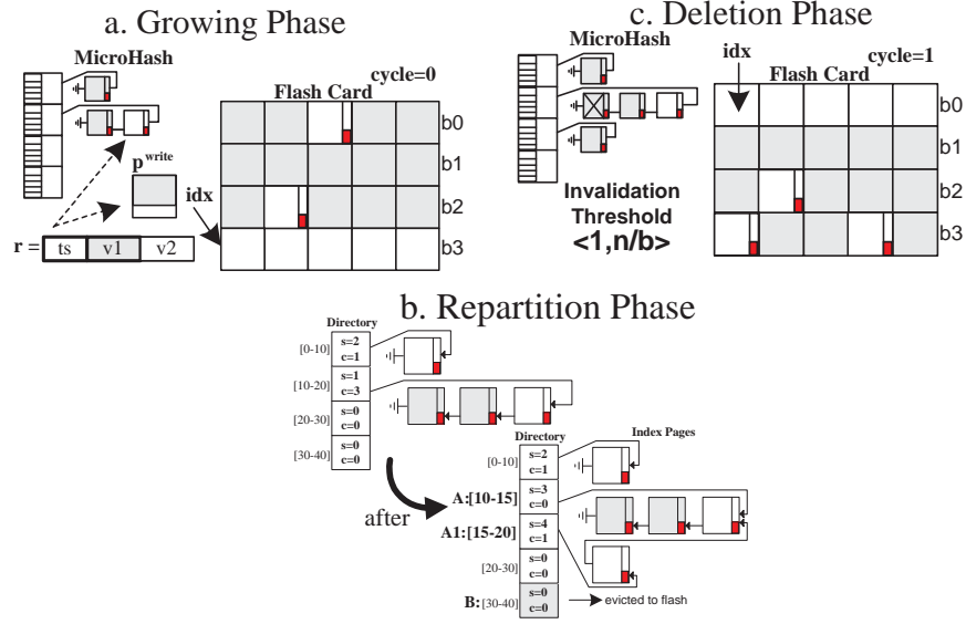
Fig. 4. The three indexing phases: a) Growing Phase, b) Repartition Phase and c) Deletion Phase
