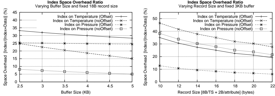
Fig. 12. Space Overhead of Index Pages with a) varying buffer size and b) varying record size.
