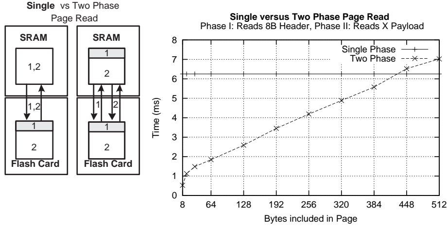
Fig. 8. a) Illustration of the Single Phase and Two Phase Page Read strategies. b) Performance comparison of the strategies on the RISE platform.
