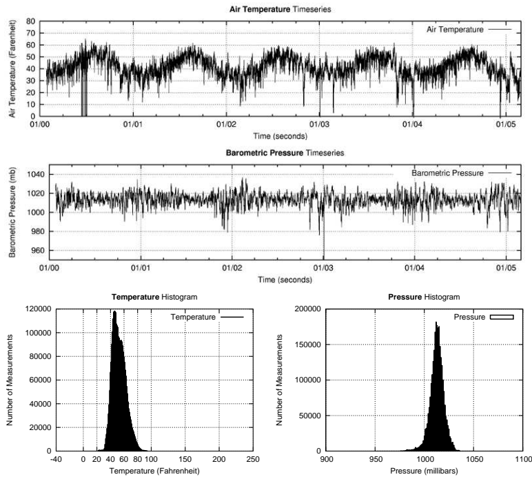
Fig. 11. Temperature (F) and Barometric Pressure (mb) readings recorded at an atmospheric monitoring site in Washington, USA. The last row indicates the respective distribution histograms for the two timeseries.
