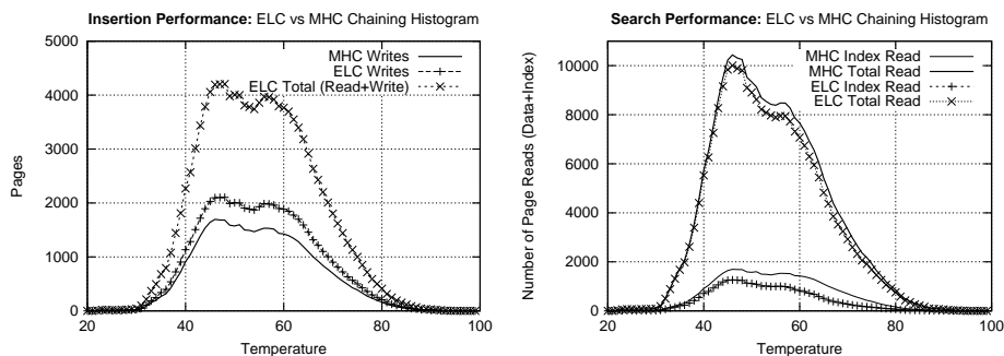
Fig. 15. Comparing MicroHash Chaining (MHC) with ELF-like Chaining (ELC) using a) Insertion Performance and b) Searching Performance by Value.
