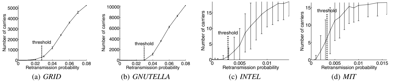
Fig. 5. Number of “residual carriers” C_{\infty} , versus the retransmission probability: The dashed vertical line marks our threshold ( s = 1 ). The information dies out below our threshold, but survives above it.
