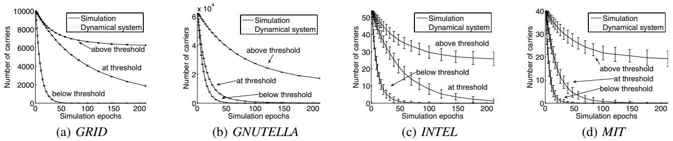
Fig. 4. Number of carriers versus time (simulation epochs): Our dynamical system (dotted lines) and simulation (solid lines). Confidence intervals show +/- one standard deviation. For each dataset we have three cases: below-, at-, and above-threshold, with parameter settings shown in Table II. Notice that (1) The dynamical system (dotted lines) is very accurate, being close to the simulation (solid lines), and (2) the number of carriers dies out very quickly below the threshold, while the information “survives” above the threshold.
