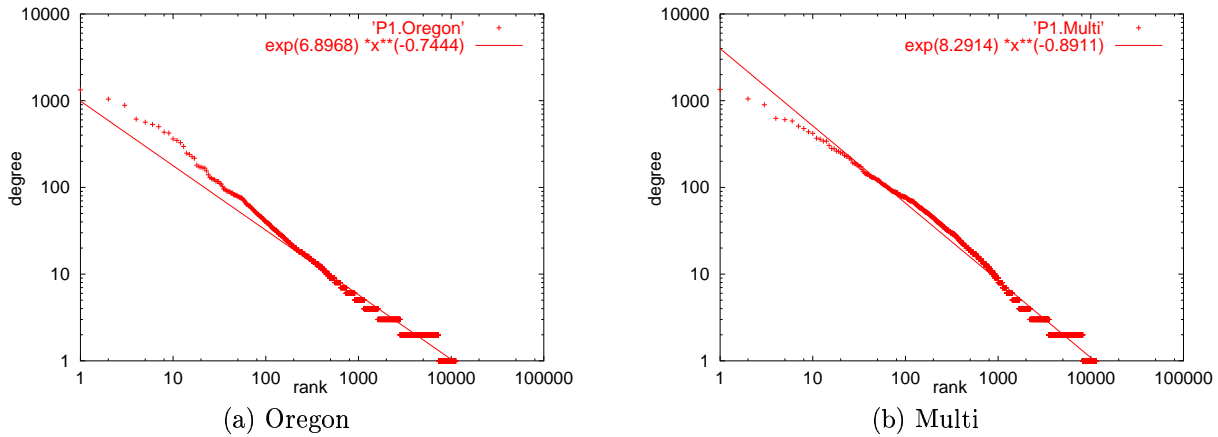
Figure 2: The rank plot. Log-log plot of the degree d_v versus the rank r_v in the sequence of decreasing degree.
