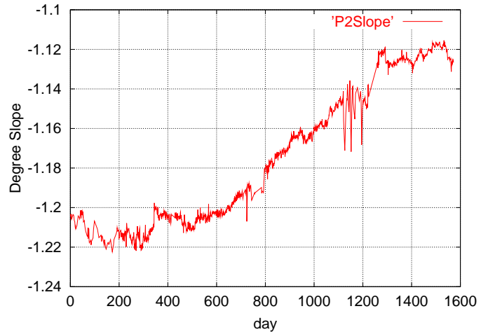
Figure 9: The evolution of the slope of the degree exponent
