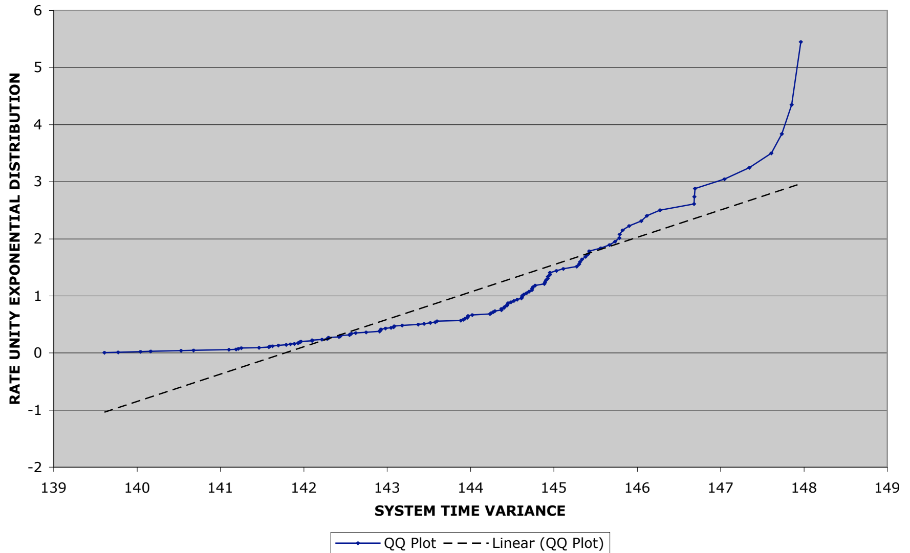
Figure 4: Q-Q Plot of Network Data vs. Exponential Distribution
