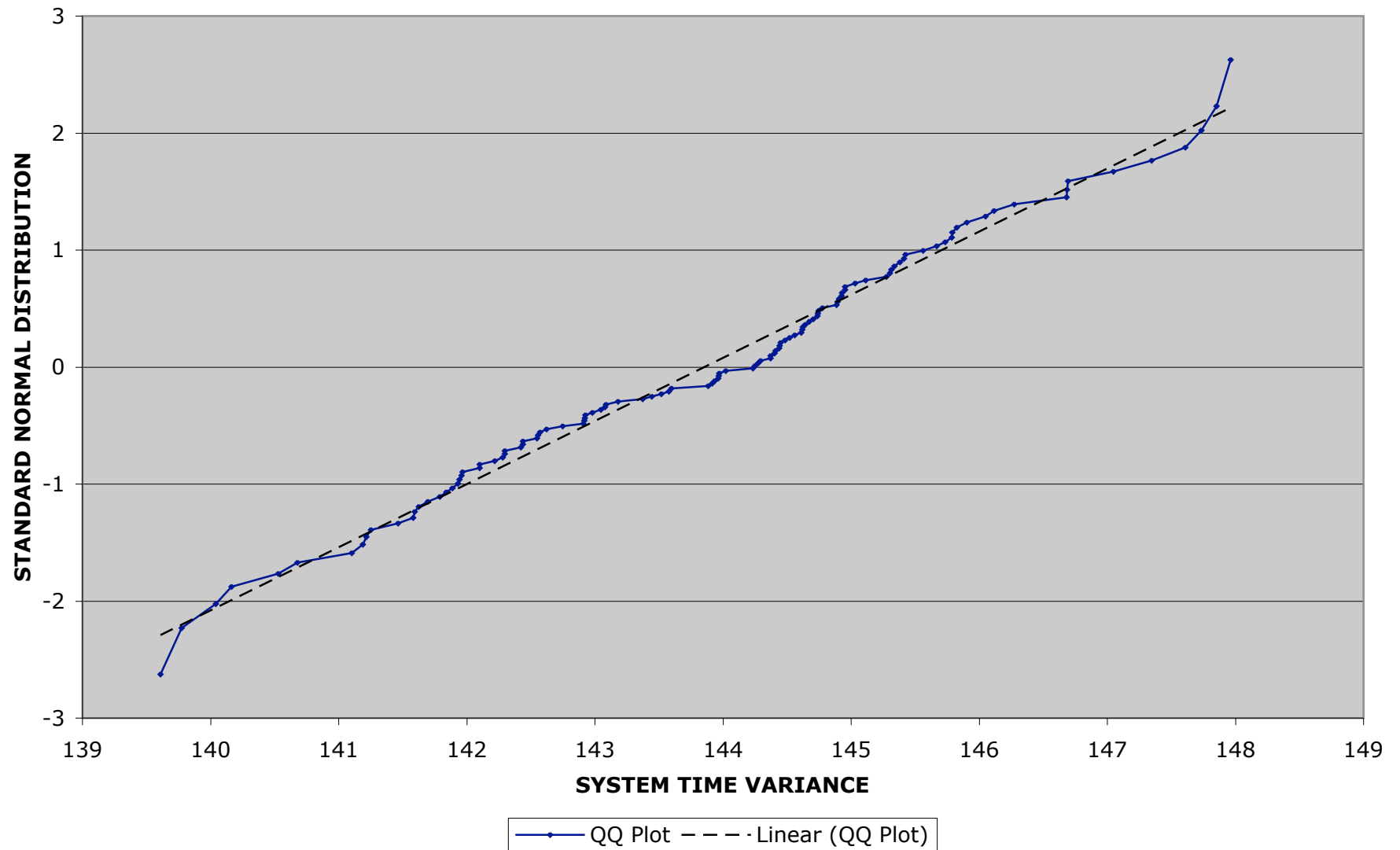
Figure 3: Q-Q Plot of Network Data vs. Normal Distribution
