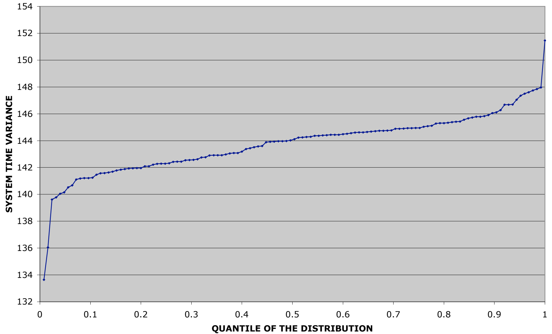
Figured 2: Sorted Network Simulation Data Gives an Inverse PDF
