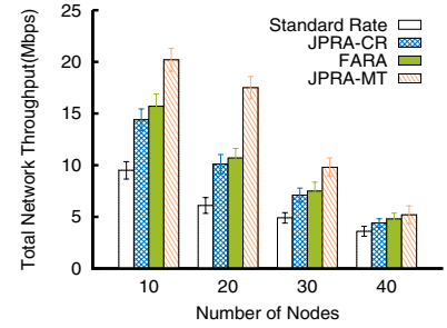
Figure 11: Network throughput with 1472 bytes packet size .
