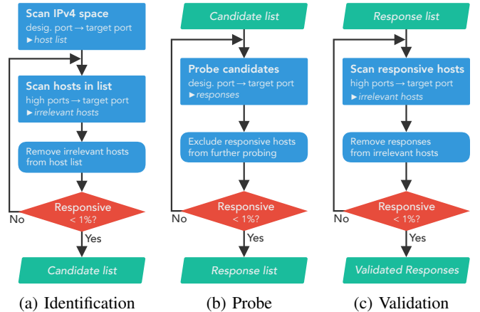
Figure 2: Three-Phase Workflow
