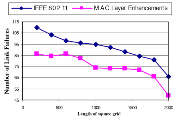
Fig. 8. Link failures in the heterogeneous network.
