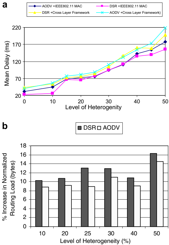
Fig. 16. End-to-end delay and routing overhead with our framework. (a) End-to-end delay. (b) Routing overhead with our cross-layer framework in the heterogeneous network.
