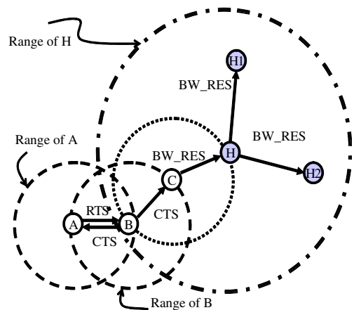
Fig. 3. CTS propagation scheme.
