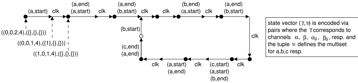
Figure 4: SDF state space of the example SDFG.
