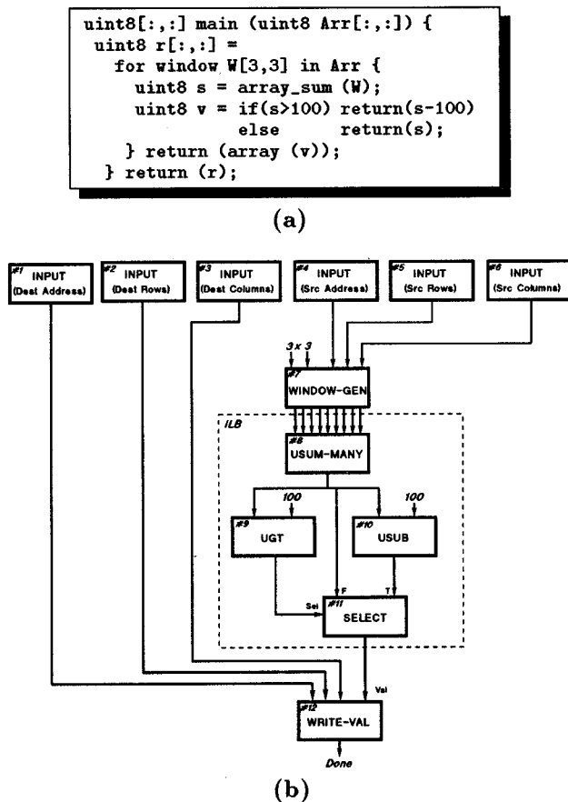
Fig. 1. (a) Simple SA-C program and (b) resulting dataflow graph.
