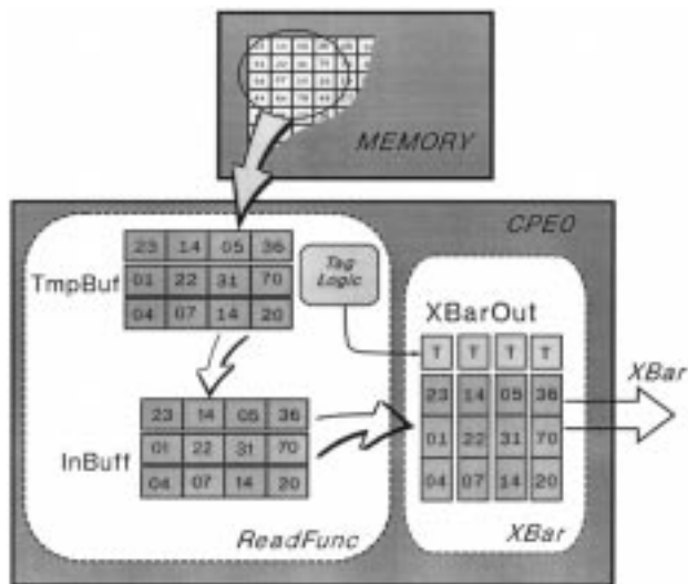
Fig. 7. Diagram of the read window generator function.
