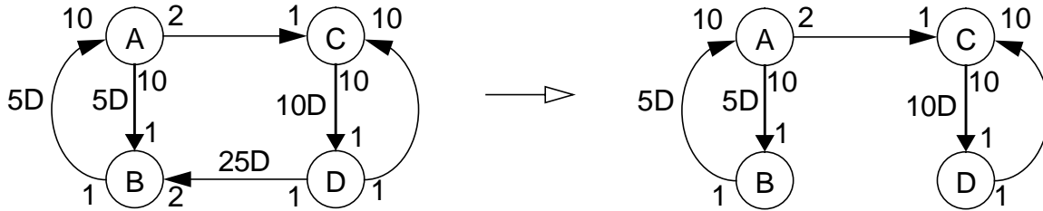
Fig. 10. An example of constructing a subindependent partition. For the strongly connected SDF graph on the left, q(A, B, C, D) = (1, 10, 2, 20) . Thus the delay on the arc directed from D to B ( 25 ) exceeds the total number of samples consumed by B in a schedule period ( 20 ). We remove this arc to obtain the new graph on the right. Since this graph is not strongly connected, a subindependent partition exists: the root strongly connected component \{A, B\} is subindependent of the rest of the graph \{C, D\} .
