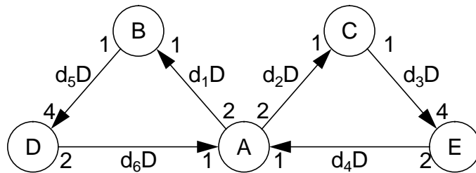
Fig. 6. An example used to illustrate the application of lemmas 1 and 2. Each d_j represents the number of delays on the corresponding arc. Here \mathbf{q}(A, B, C, D, E) = (2, 4, 4, 1, 1) .
