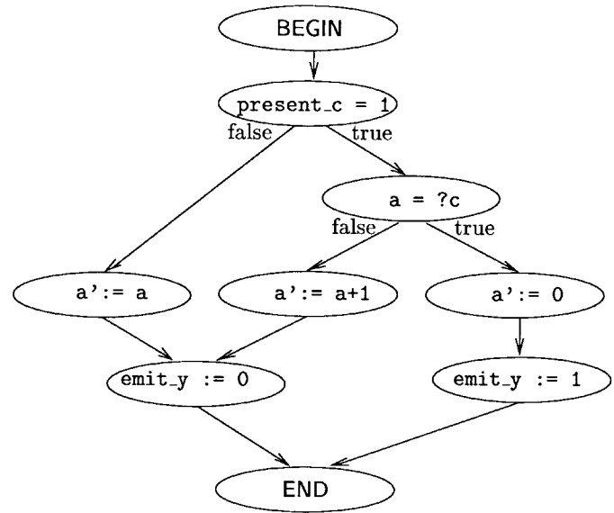
Fig. 1. A simple s-graph.
