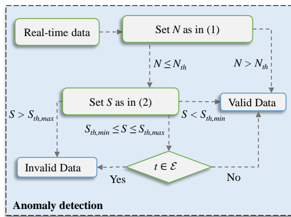
Fig. 3. Outline of the proposed anomaly detection method.
