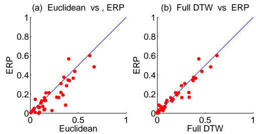
Figure 13: Accuracy of ERP, above the line Euclidean/Full DTW outperforms ERP
