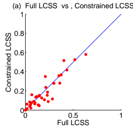
Figure 14: Accuracy of Constrained LCSS, above the line Full LCSS outperforms Constrained LCSS
