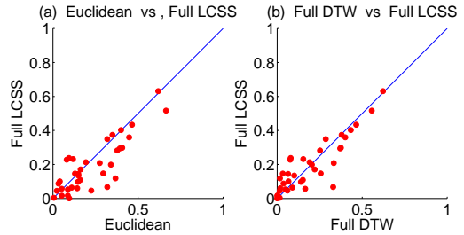
Figure 11: Accuracy of LCSS, above the line Euclidean/Full DTW outperforms Full LCSS
