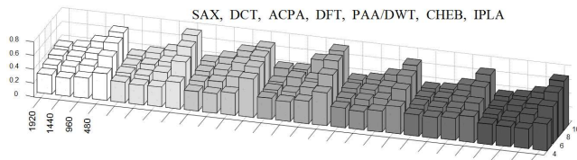
Figure 3: The tightness of lower bounds for various time series representations on an ECG data set
