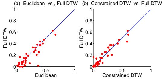
Figure 8: Accuracy of DTW, above the line Euclidean/Constrained DTW outperforms Full DTW
