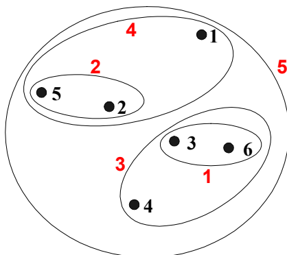
Nested Clusters
