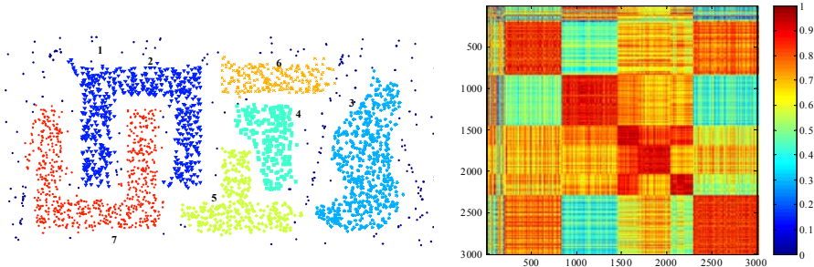
DBSCAN
