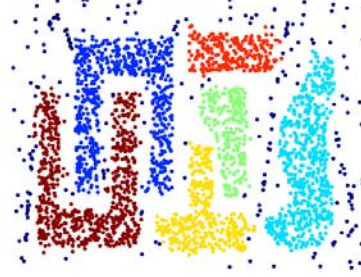
Clusters
