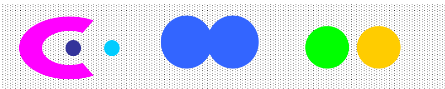
6 density-based clusters
