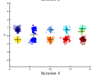
Iteration 4
