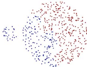
Two Clusters
