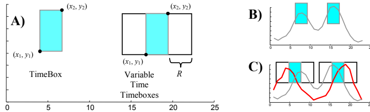
Fig. 5. A Timebox may be visualized as a shaded rectangle through which a qualifying sequence must pass. In contrast, an Variable Time Timeboxes (VTT) requires a qualifying sequence to have its value within the shaded region, allowing the shaded region to move anywhere within the larger constraining rectangle (A). Unlike Timeboxes (B), VTTs are able to detect patterns with a degree of uncertainty in the time axis
