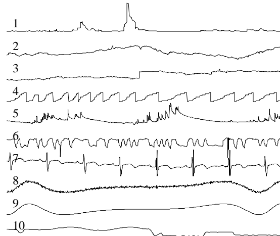
Figure 3. The ten datasets used in the experiments. 1) Radio Waves. 2) Exchange Rates. 3) Tickwise II. 4) Tickwise I. 5) Water Level. 6) Manufacturing. 7) ECG. 8) Noisy Sine Cubed. 9) Sine Cube. 10) Space Shuttle
