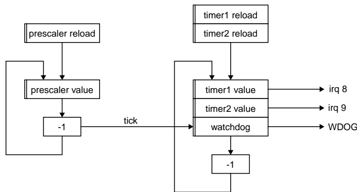
Figure 19: Timer unit block diagram
