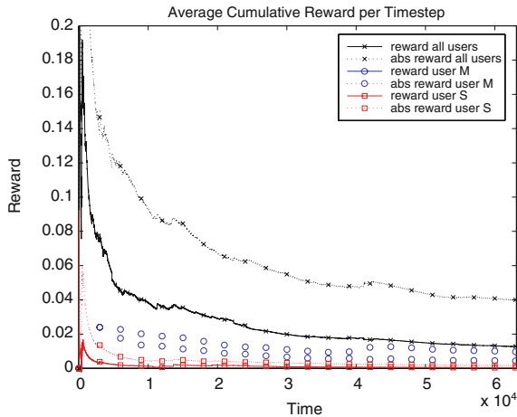
Fig. 6 The average reward received by Cobot over time. The x-axis represents sequential Cobot-initiated RL actions for which it has received at least one reward or punishment event. The y-axis indicates the average cumulative reward received up to each such action. We examine both total reward (in which we sum the positive and negative values received), as well as absolute total reward (in which we ignore sign and simply count the total amount of feedback). We plot these quantities both over all users, and for two particular users we call Users M and S. In all cases, as time progresses, Cobot is receiving less feedback. This occurs despite the fact that Cobot is learning policies that coincide with the preferences of Users M and S, suggesting that this may not be a useful measure of performance
