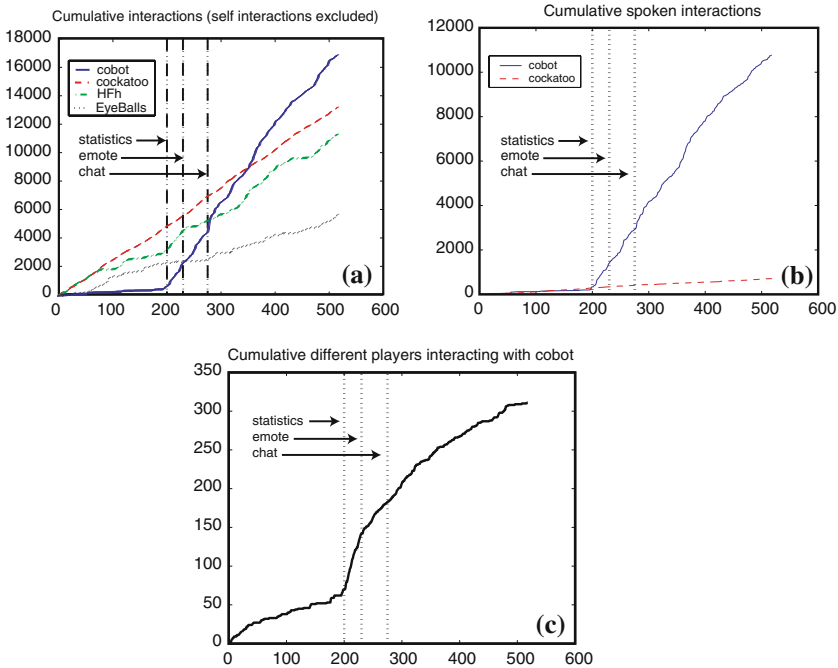
Fig. 3 Cumulative interactions with objects in the Living Room. (a) Cumulative number of verbs (speech verbs, hugs, waves, etc.) directed towards various Living Room denizens: Cobot, the Cockatoo, and the two human users most interacted with during this period. The x-axis measures cumulative events (in thousands) of any type in the Living Room, while the y-axis measures cumulative events directed at the indicated user. Each dashed vertical line indicates the introduction of a major new feature (from the left, his social statistics, his emoting abilities, and his extended chat abilities). A straight line—such as the Cockatoo’s—indicates constant interaction. By contrast, Cobot’s curve shows sudden changes in the slope coinciding with new features. Note that even when the slope levels off afterwards, it remains higher than it was previously, indicating long-term impact. Judging from cumulative interaction, Cobot is the most popular user in the Living Room. (b) Cumulative speech acts directed at Cobot and the Cockatoo. Clearly users interact with the two artifacts differently. Most of the interaction with Cockatoo is explained by users invoking its gag verb to silence it. Still, note that there is constant non-zero daily spoken interaction with it as well, indicating that users are willing to talk to even such a relatively simple creature. Also, note that before his new abilities surfaced, Cobot enjoyed a comparable amount of spoken interaction. (c) Variety of users interacting with Cobot. Over time, users brought others into the Living Room to play with him. Also, users who were already in the Living Room but ignoring Cobot began interacting with him when they saw others using his abilities
