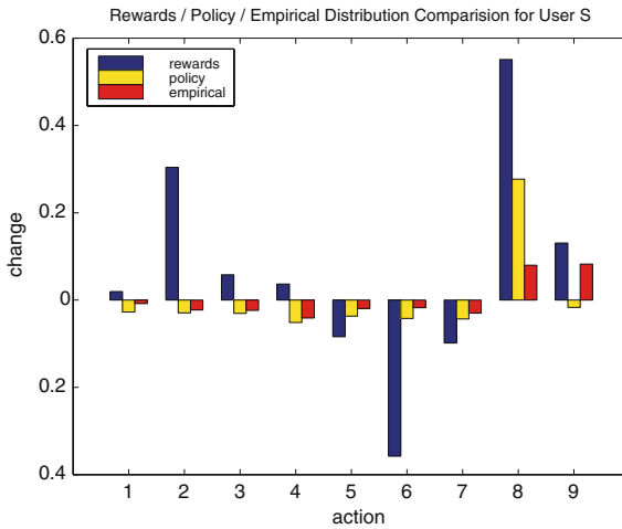
Fig. 8 Rewards received, policy learned, and effect on actions for User S. Same as Figure 7, but for User S. While not as visually compelling as the data for User M, the quantitative agreement between the orderings is again very strong
