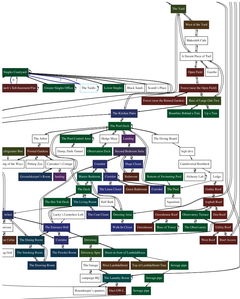
Fig. 2 Physical map. A partial map of LambdaMOO. Nodes are rooms, and directed edges indicated exits from one room to another. Colors reflect a basic similarity between nodes based purely on the text for the room’s description. Cobot has visited over 1667 rooms in his lifetime. There is an entire sub part of LambdaMOO called the RPG—a place where role playing games occur—that cobot has never explored
