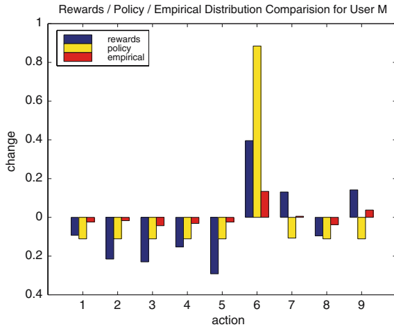
Fig. 7 Rewards received, policy learned, and effect on actions for User M. For each of the nine RL actions, three quantities are represented. The blue bars (left) show the average reward given by User M for the corresponding action. The average reward given by User M across all actions has been subtracted off, so that “positive” bars indicate a relative preference for that action by User M, and “negative” bars indicate a relative objection to that action. The yellow bars (middle) show the policy (probability distribution) learned by Cobot for User M. The probability assigned to each action in the uniform distribution ( 1/9 ) has been subtracted off, so again the bars indicate relative preferences and objections of the learned policy. The red bars (right) show, for each action, the empirical frequency with which that action was taken by Cobot when User M was present, minus the empirical frequency to which the presence of User M biases Cobot’s behavior towards M’s preferences. We see that (a) the policy learned by Cobot for User M aligns nicely with the preferences expressed by M through her training (comparison of left and middle bars), and (b) Cobot’s behavior shifts strongly towards the learned policy for User M whenever she is present (comparison of middle and right bars). The actions are presented here in the same order as in Table 6.4. To go beyond a qualitative visual analysis, we have defined a metric that measures the extent to which two orderings of actions agree. Briefly, given two sequences of actions we count elementwise disagreements. When two elements within a sequence have the same value (and so could be swapped) we choose the ordering that minimizes that sequence’s disagreement with the other. We also extend this to allow for nearly-equal values. The agreement between the action orderings given by the rewards of User M and the policy learned for User M are near-perfect by this measure, as are the orderings given by the policy and the empirical distribution of rewards
