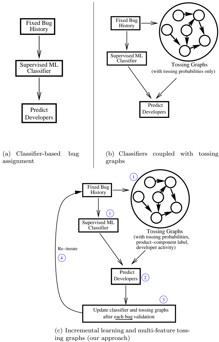
Figure 7: Comparison of bug assignment techniques.
