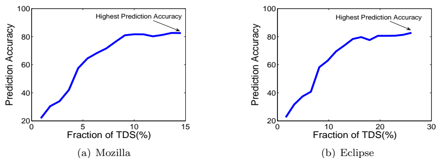
Figure 11: Change in prediction accuracy when using subsets of bug reports using Naïve Bayes classifier.
