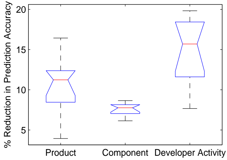
(a) Mozilla
