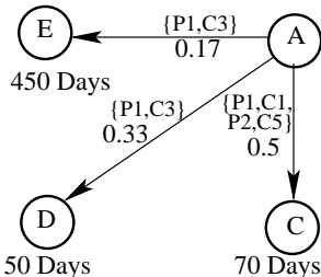
Figure 5: Multi-feature tossing graph (partial) derived from data in Table 2.
