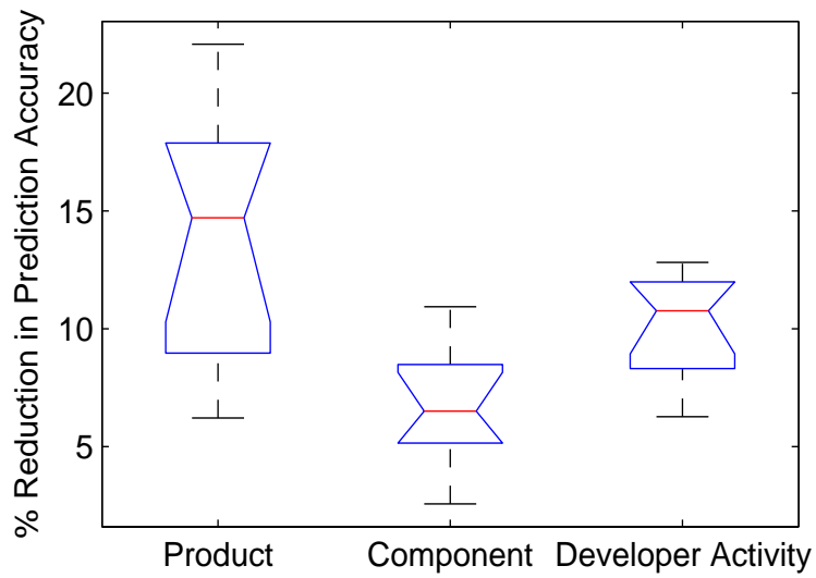
(b) Eclipse
