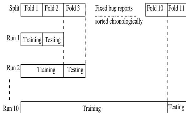
Figure 2: Folding techniques for classification as used by Bettenburg et al.
