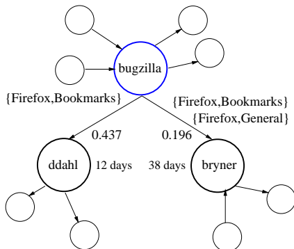
Figure 6: Actual multi-feature tossing graph extracted from Mozilla.
