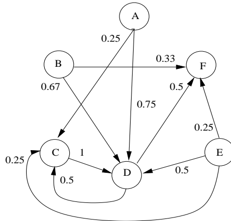
Figure 3: Tossing graph built using tossing paths in Table 1.
