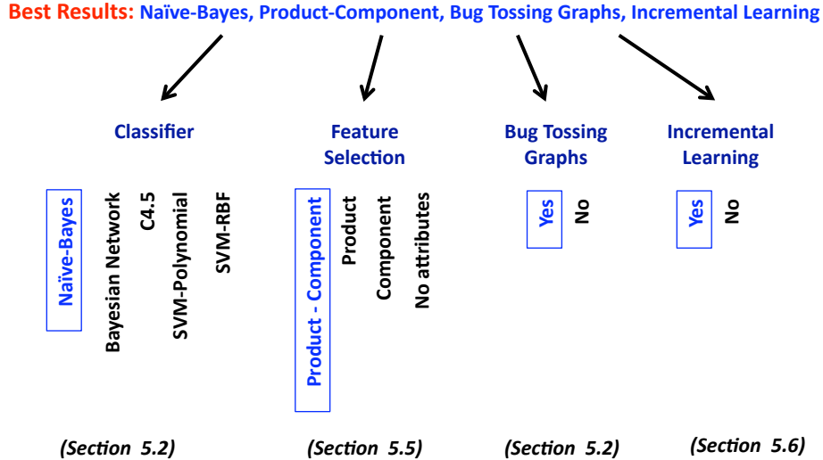
Figure 1: Overview our approach to ablative analysis for automating bug assignment: best case (boxed vertical text), attributes varied (unboxed vertical text), and the corresponding sections where the attributes and their importance are discussed.
