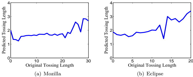
Figure 9: Average reduction in tossing lengths for correctly predicted bugs when using ML + Tossing Graphs (using both classifiers).
