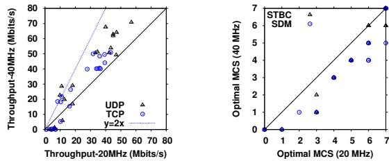
Figure 6: Throughput experiments (a) with rate control and (b) with fixed rates.
