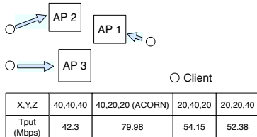
Figure 11: ACORN provides the highest throughput in settings with interference. X, Y, Z denote the channel widths (MHz) used by APs 1, 2 and 3.
