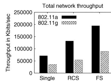
Fig. 2. Comparison between FS in isolation, RCS, and single channel selection, for 802.11a as well as 802.11g.
