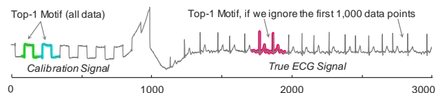
Figure 1: blue/fine: A snippet of ECG data from the LTAF-71 Database [13]. The top motifs come from regions of the calibration signal because they are much more similar than the motifs discovered if we search only data that contains true ECGs.
