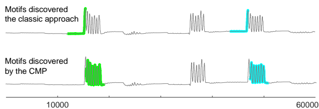
Figure 18: By correcting the matrix profile with an AV using the algorithm in Table 3, we discover the true motifs of finger flexion pattern.
