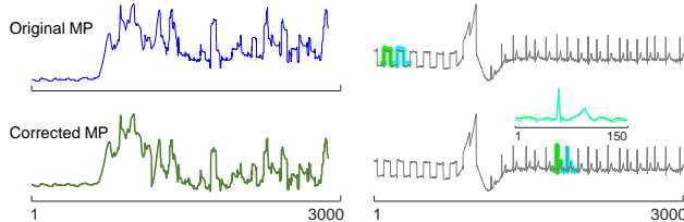
Figure 14: By correcting the MP to bias away from stop-word motifs, we can discover medically meaningful motifs.
