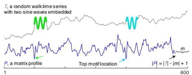
Figure 4: A time series T and its self-join matrix profile P .
