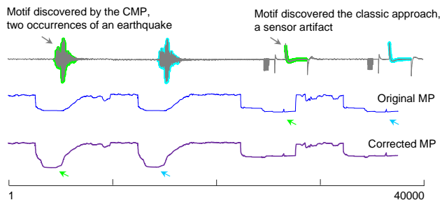
Figure 19: The top motif returned by the classic approach is not an earthquake, but a sensor artifact . Using guided motif search framework, we can avoid such various misleading sensor artifacts, which swamp this 17,279,800 data-points earthquake dataset. The time series shown was edited for visual clarity.
