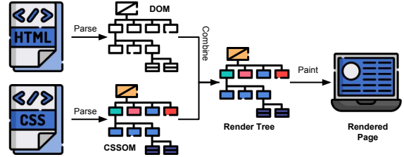
Figure 3: Rendering Path for Blink
