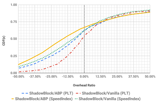
Figure 7: CDF for performance metrics
