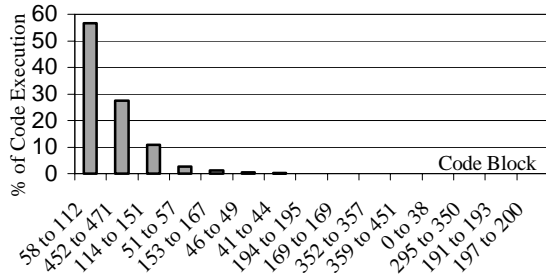
Figure 4: A few loops often comprise most of an application’s execution time, as in the matrix multiply example.
