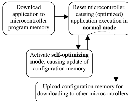
Figure 3: Self-optimization methodology.
