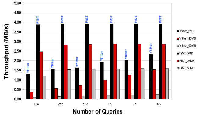
Fig. 13. Throughput of FiST and YFilter when using 5, 25, and 50MB XML documents, and queries for dataset 2 (10% occurrence of ‘//’ and ‘*’ in the queries).
