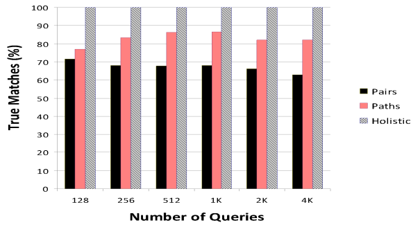
Fig. 11. The percentage of true matches as reported from several hardware approaches.
