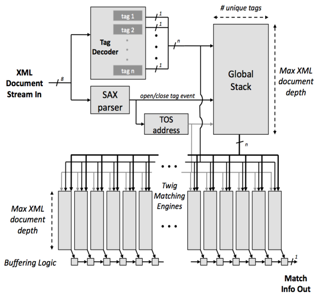
Fig. 4. High-Level XML Filtering System.
