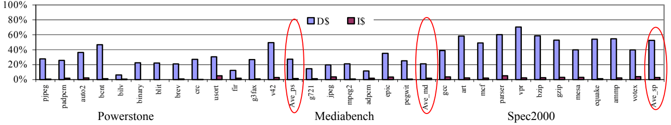
Figure 3: Tag address change frequency of data and instruction cache.
