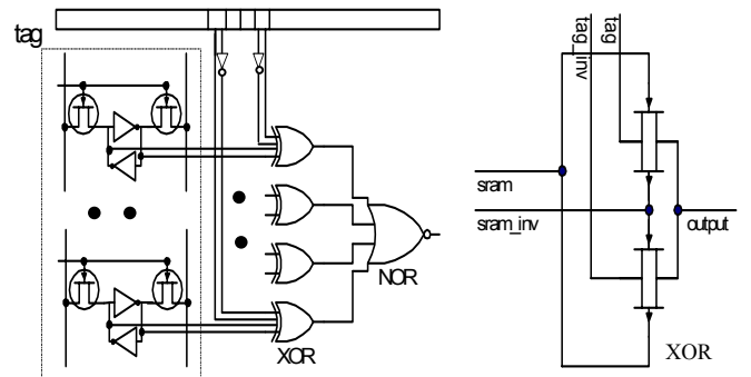
Figure 4: Design of a fully associative memory for the halt tag array, based on a static circuit only. The sixteen input static comparator is composed of four XOR gates and one NOR gate. Eight inputs come from the SRAM cells that store the halt tag, while the other eight inputs come from the desired address' least four-tag bits.
