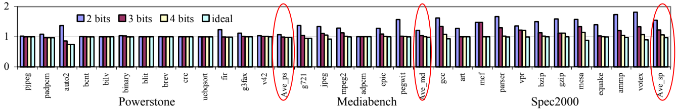
Figure 2: Average number of ways of instruction cache activated when 2-bit, 3-bit, and 4-bit are compared in parallel with address decoder. Ave_ps , Ave_md , and Ave_sp stand for average of Powerstone, Mediabench, and Spec 2000 respectively.
