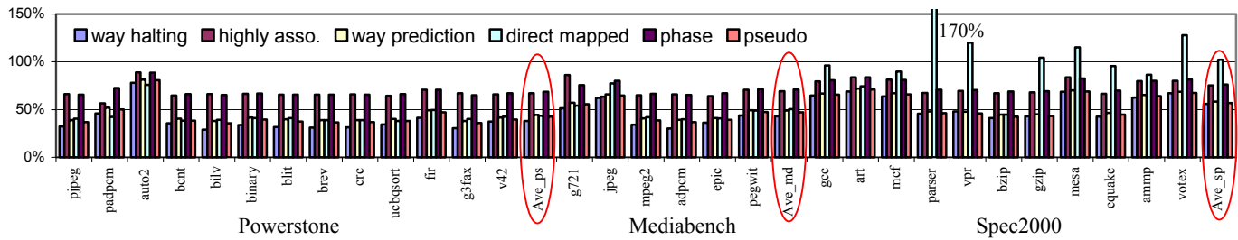
Figure 5: Energy for various cache designs, for Powerstone benchmarks, normalized to a conventional 4-way cache.
