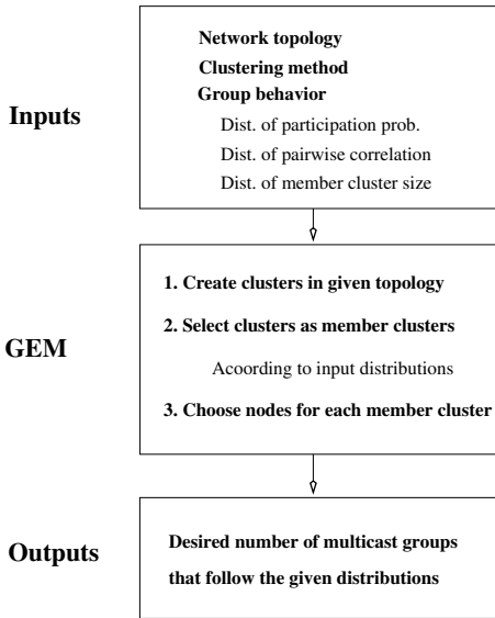
Figure 12: An illustration of GEM.
