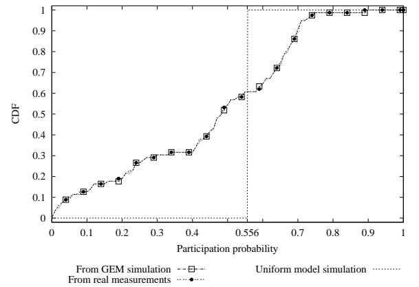
Figure 14: The comparison of group participation probability distribution of clusters for IETF43-Video between measurement and modelling data (GEM and Uniform model).
