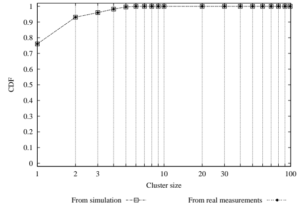
Figure 13: The comparison of cluster size distribution for IETF43-Video between measurement and modelling data.
