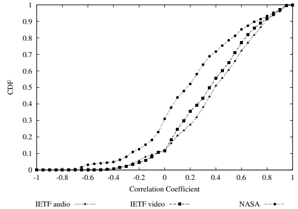
Figure 8: CDF of the correlation coefficient of clusters for data sets from MBONE (real data).
