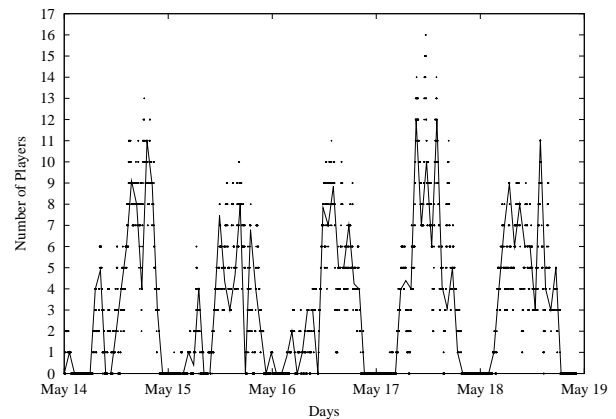
Figure 4: The data set sampled from net game server 1 (QS-7).
