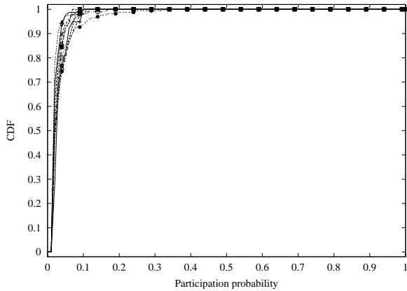
Figure 7: CDF of the participation probability of nodes for data sets from net games (including 10 data sets).
