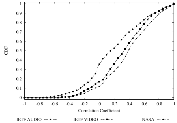
Figure 11: CDF of the correlation coefficient of nodes for data sets from MBONE (real data).
