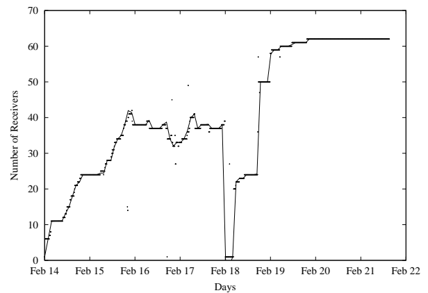
Figure 3: The data set sampled from NASA Shuttle Lunch (NASA).
