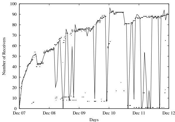
Figure 1: The data set sampled from IETF Meeting Audio (IETF43-A).
