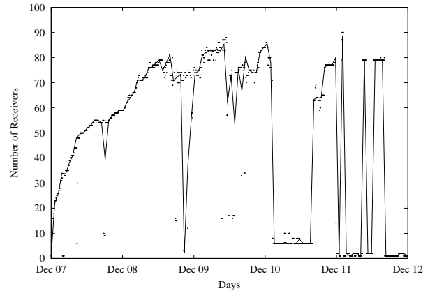
Figure 2: The data set sampled from IETF Meeting Video (IETF43-V).
