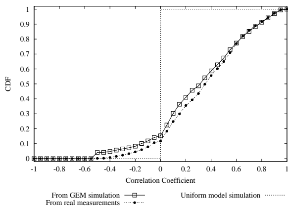
Figure 15: The comparison of correlation coefficient distribution of clusters for IETF43-Video between measurement and modelling data (GEM and Uniform model).
