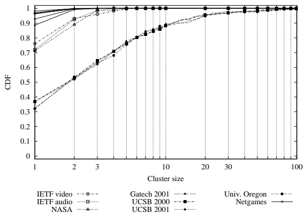
Figure 5: CDF of cluster size for data sets from MBONE and net games. The upper set of curves are for net game data sets (with 5 game servers providing IP addresses of players), the middle set of curves are for MBONE real data sets (IETF43-A, IETF43-A, and NASA), and the lower set of curves are for MBONE cumulative data sets.
