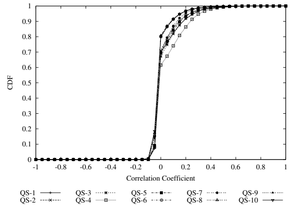
Figure 9: CDF of the correlation coefficient of nodes for data sets from net games (including 10 data sets).
