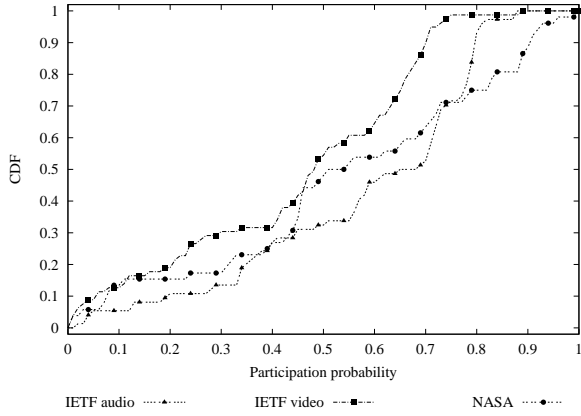
Figure 6: CDF of the participation probability of clusters for data sets from MBONE (only real data).
