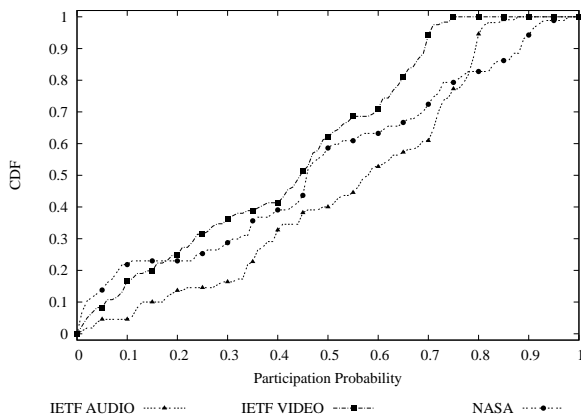
Figure 10: CDF of the participation probability of nodes for data sets from MBONE (only real data).
