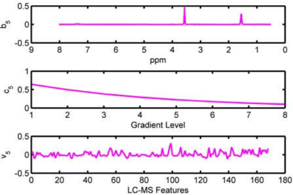
Figure 1(e) (e) Component 5: Propanol
