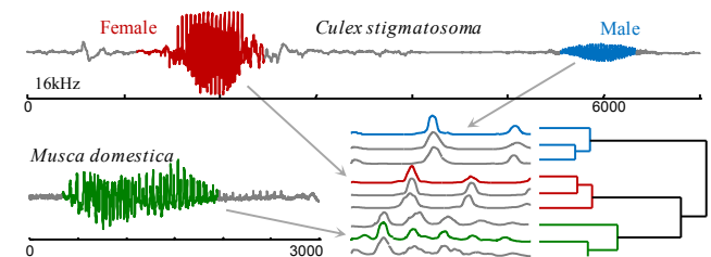
Figure 11: top) An audio snippet of a female Cx. stigmatosoma pursued by a male. bottom left) An audio snippet of a common house fly. bottom right) If we convert these sound snippets into periodograms we can cluster and classify the insects.
