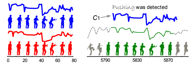
Figure 10: left) A query shown to the user during a run on the activity dataset; the teacher labeled it Pushing and a new concept C_1 was added to the dictionary. right) About 9.6 minutes later, the classifier detected a new example of the class.
