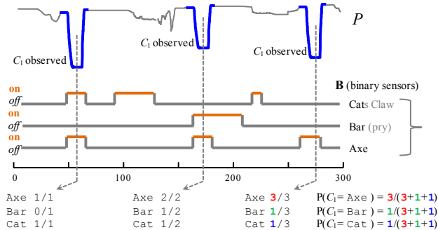
Figure 9: An illustration of a weak teacher. top) A stream P in which we detect three occurrences of the pattern C_1 . middle) At the time of detection we poll a set of binary sensors to see which of them are active. bottom) We can use the frequency of associations between a pattern and binary “votes” to calculate probabilities for C_1 ’s class label.
