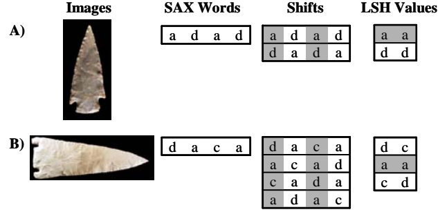
Figure 14: The same two images as in Figure 13 are both mapped to LSH value “aa”. Here w = 4 , \Sigma = \{a, b, c, d\} , and k = 2 . The indices chosen by the hash function are \{1, 3\}
