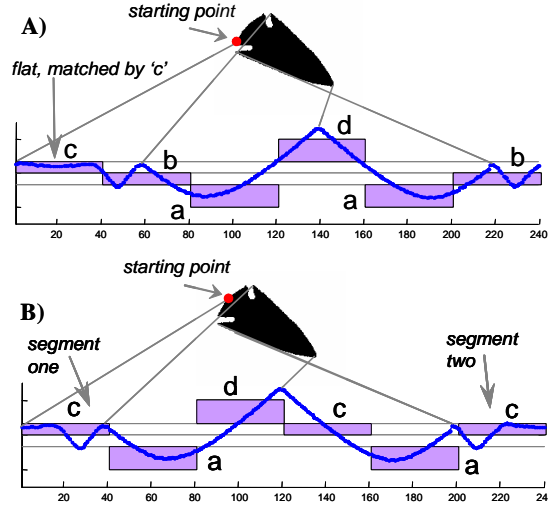
Figure 12: An arrowhead image is converted to time series starting from two different points. Top ) The first SAX symbol c approximates the first 40 data points perfectly. Bottom ) However the same plateau time series is divided into two parts (the first and last segments of the time series)
