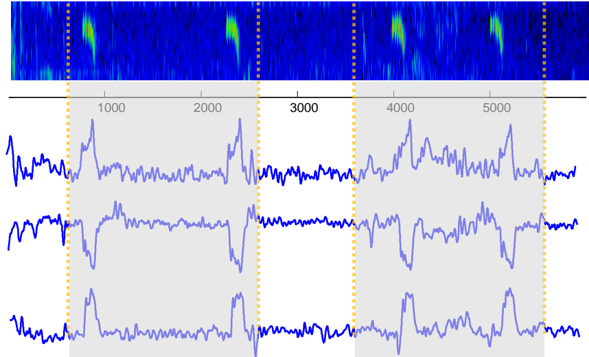
Fig.4 Three coefficients from the MFCC space of a Southern Chestnut-Tailed Antbird ( Myrmeciza hemimelaena ). This bird’s call is typically transcribed as “ klee-klee ” [11]; thus, the above shows two calls, the second being significantly briefer.
