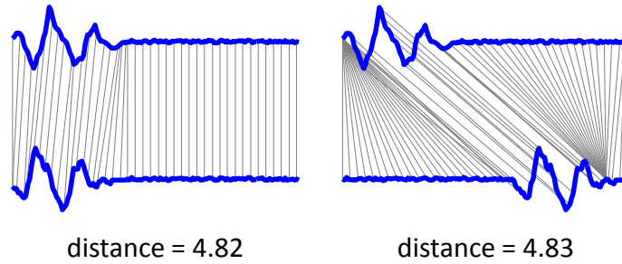
Fig.6 For the one-dimensional case, adding lag to one of the time series can change the warping drastically, without changing the distance by a significant amount.
