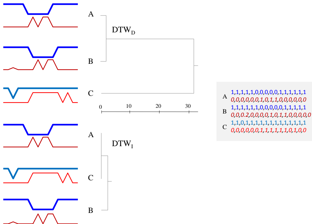
Fig.10 Three 2-dimensional time series (raw values shown in inset) single-linkage hierarchically clustered using DTW_D (top) and DTW_I (bottom). Here DTW_D produces an intuitive clustering, closely linking A and B, whereas DTW_I uses its greater representational flexibility to produce a bizarre result, finding A to be identical to C.
