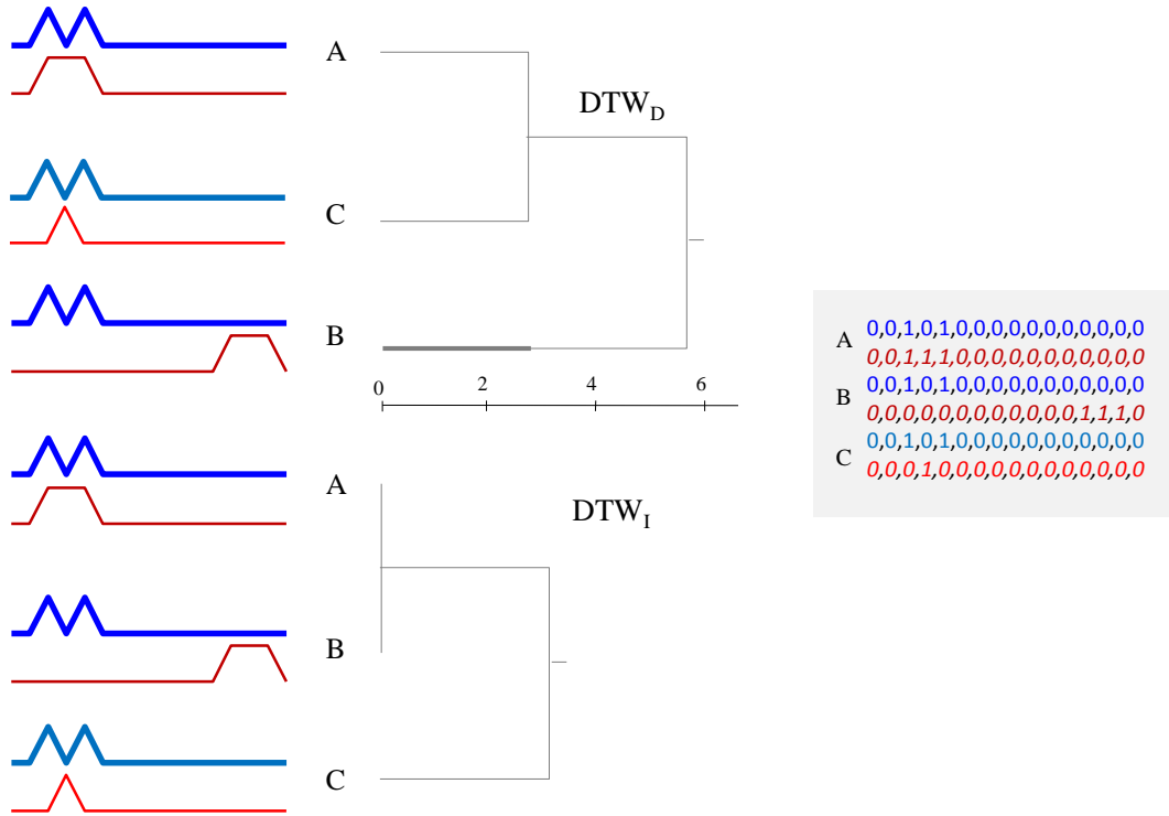
Fig.11 Three 2-dimensional time series (raw values shown in inset) single-linkage hierarchically clustered using DTW_D (top) and DTW_I (bottom). Here DTW_I produces an intuitive clustering, closely linking A and B, whereas DTW_D uses only one warping path to measure distances therefore producing a bizarre result, finding A to be identical to C. Compare to Fig.10 .
