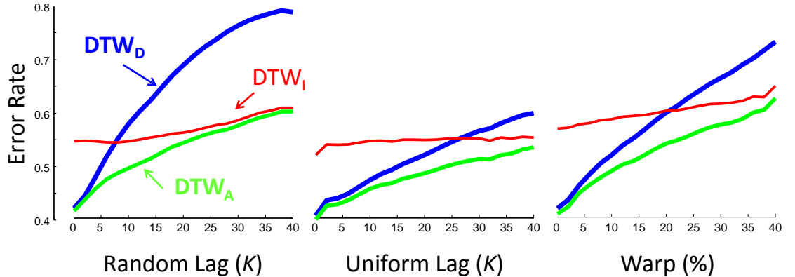
Fig.18 The experiments shown in Fig.7 , Fig.8 and Fig.9 , revisited using the DTW A technique.
