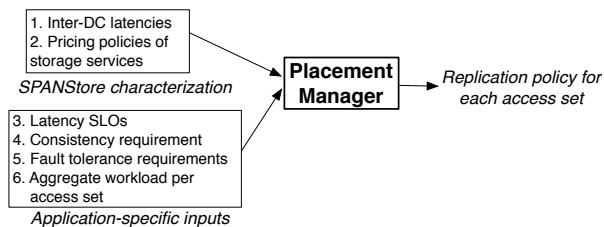
Figure 3: Overview of PMan 's inputs and output.
