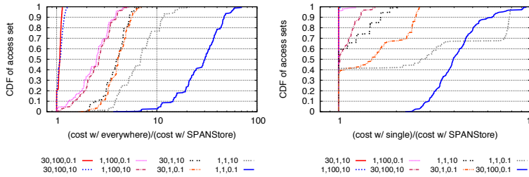
Figure 11: Cost savings enabled by SPANStore compared to Everywhere (left) and Single (right) replication policies. Legend indicates GET:PUT ratio, average object size (in KB), and overall data size (in TB).
