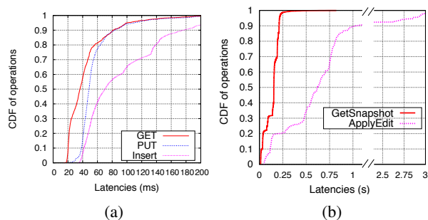
Figure 14: CDF of operation latencies in (a) Retwis and (b) ShareJS applications.
