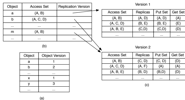
Figure 7: At any data center A , SPANStore stores an (a) in-memory version mapping for objects stored at A . If the application is deployed at A , SPANStore also stores (b) the access set mapping for objects whose access set includes A , and (c) replication policy versions for different epochs.
